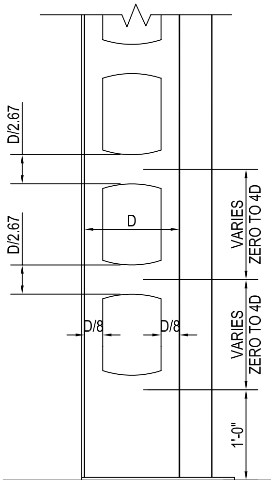
HI-SPAN TRUSS HOLE PATTERN LAY-OUT
