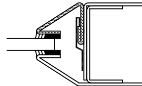
SNAP-ON BEVELED GLASS STOP
