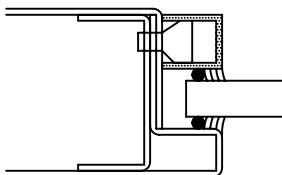
ALUMINUM SNAP-ON GLASS STOP
