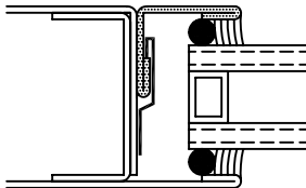
SNAP-ON GLASS STOP
